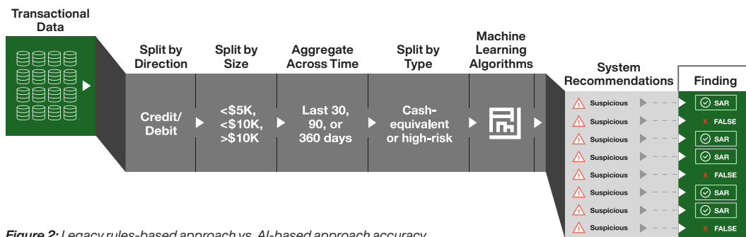
Figure 2: Legacy rules-based approach vs. AI-based approach accuracy
