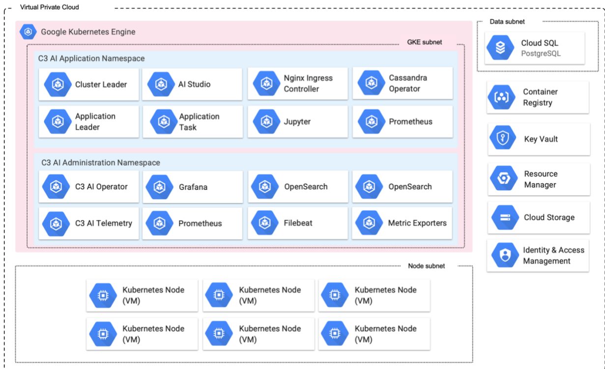
Figure 2. GCP Architecture with C3 AI Platform Deployment
