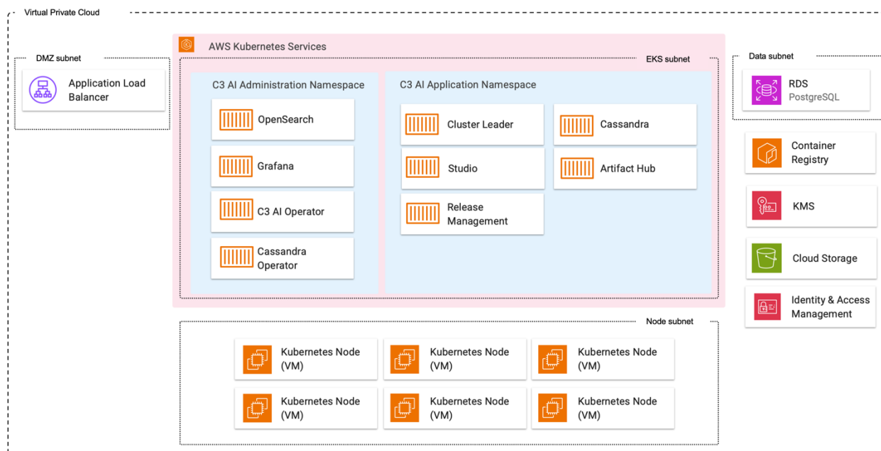
Figure 2. AWS Architecture with C3 Agentic AI Platform Deployment
